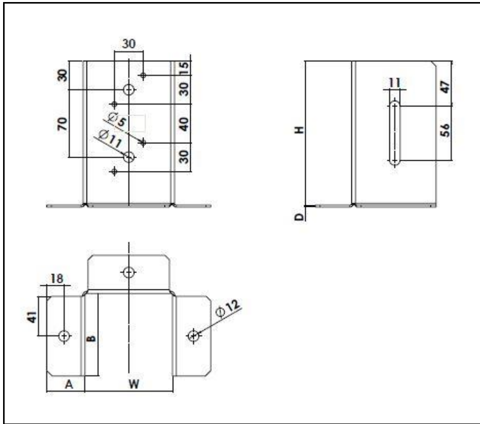
Figure 10 Type PSP DX 90
