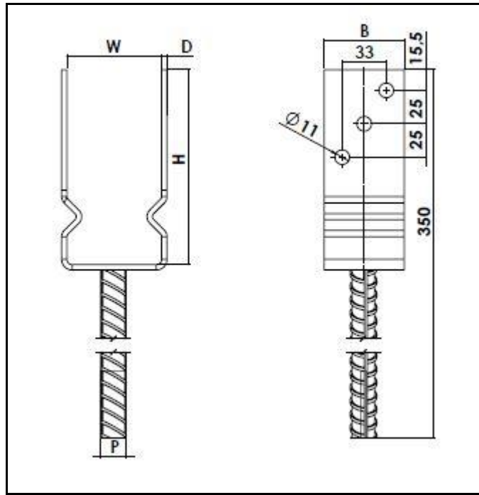
Figure 13 Type PSZ 70
