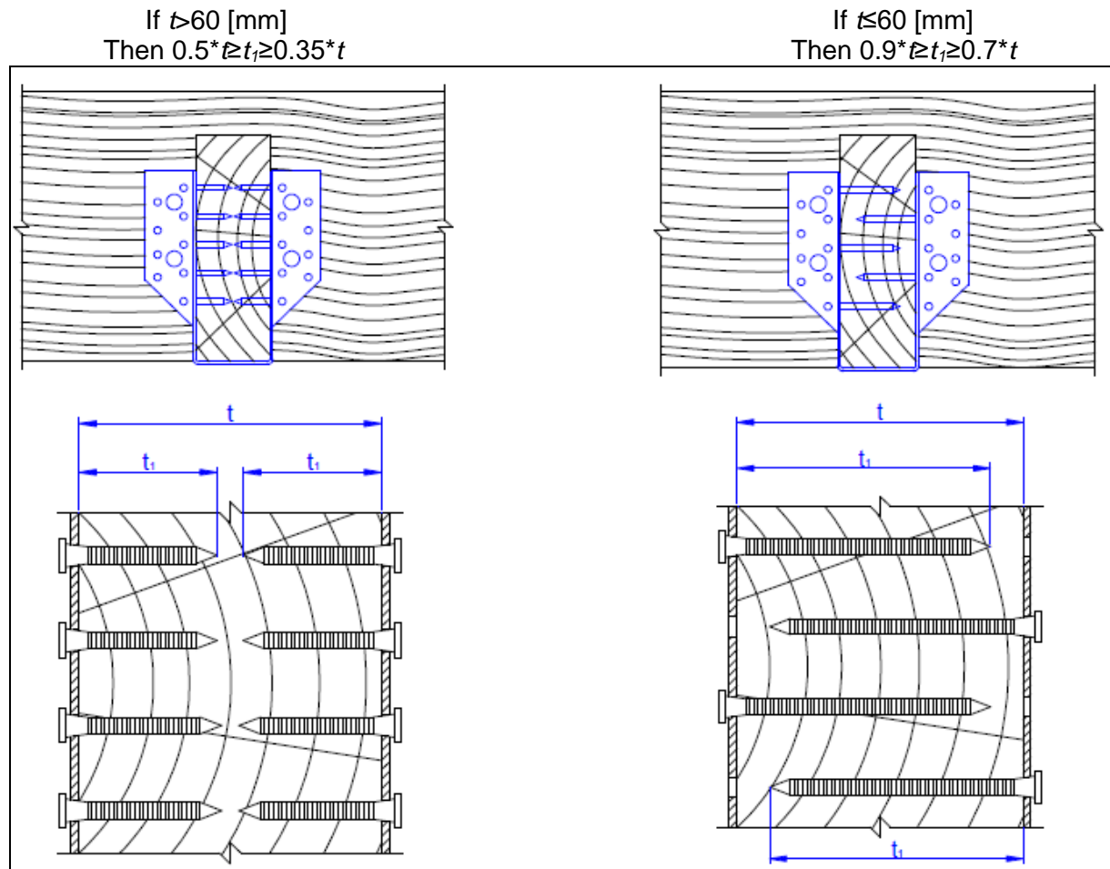
Figure 61 Rule for placement nails
