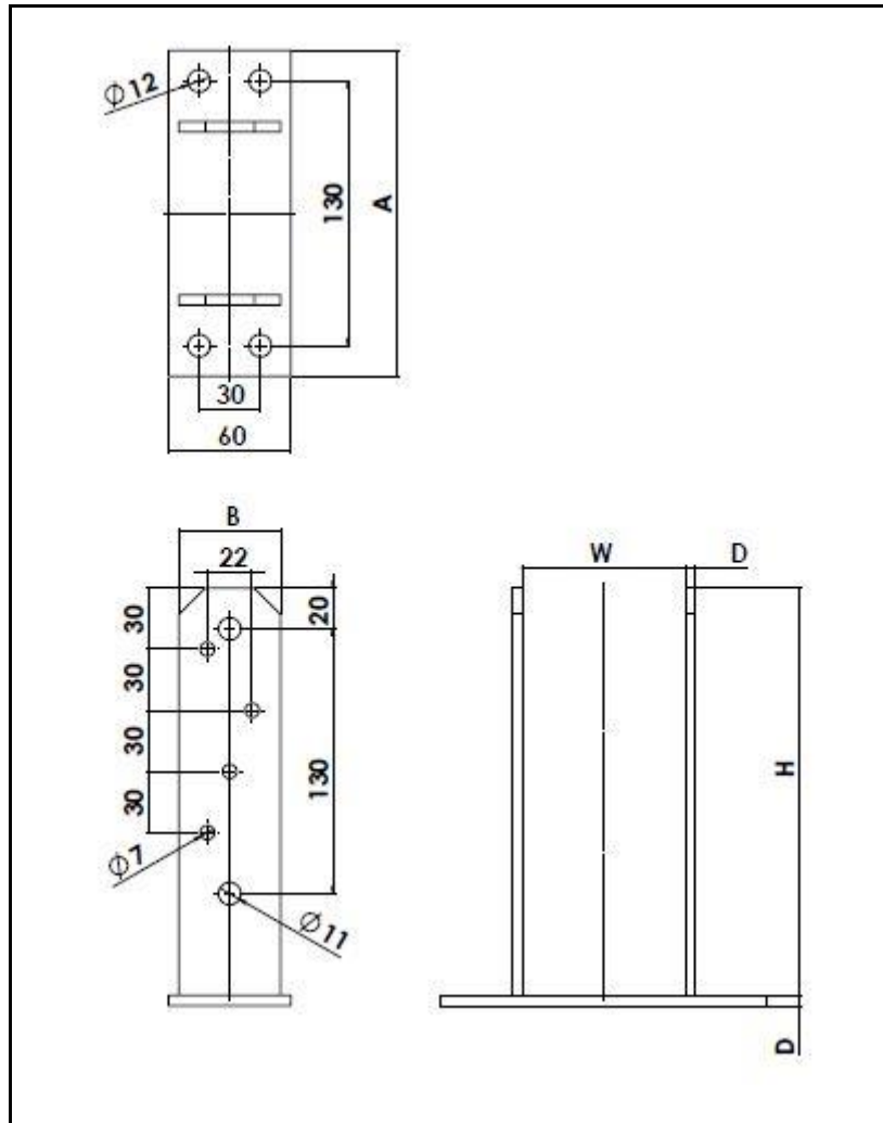
Figure 11 Type PST 80
