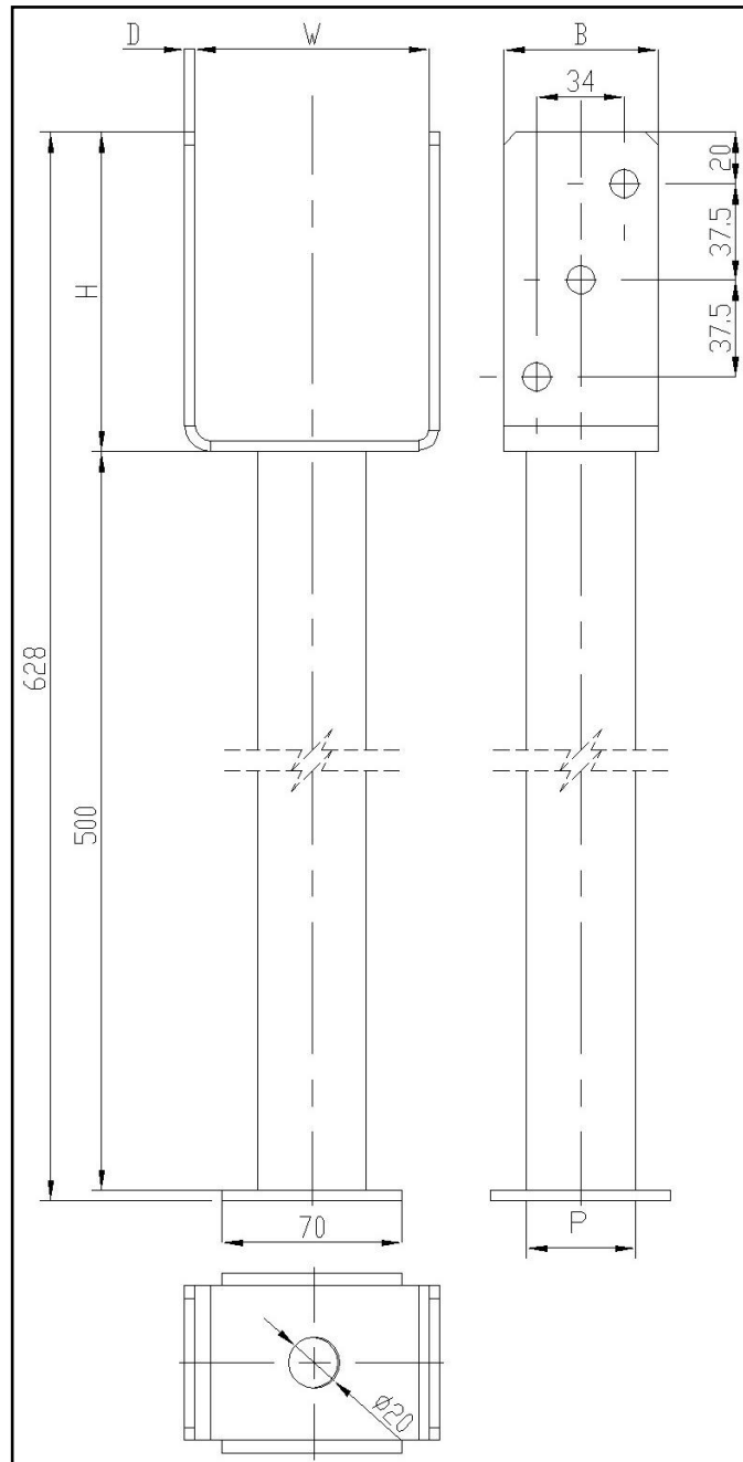
Figure 28 Type PS R500
