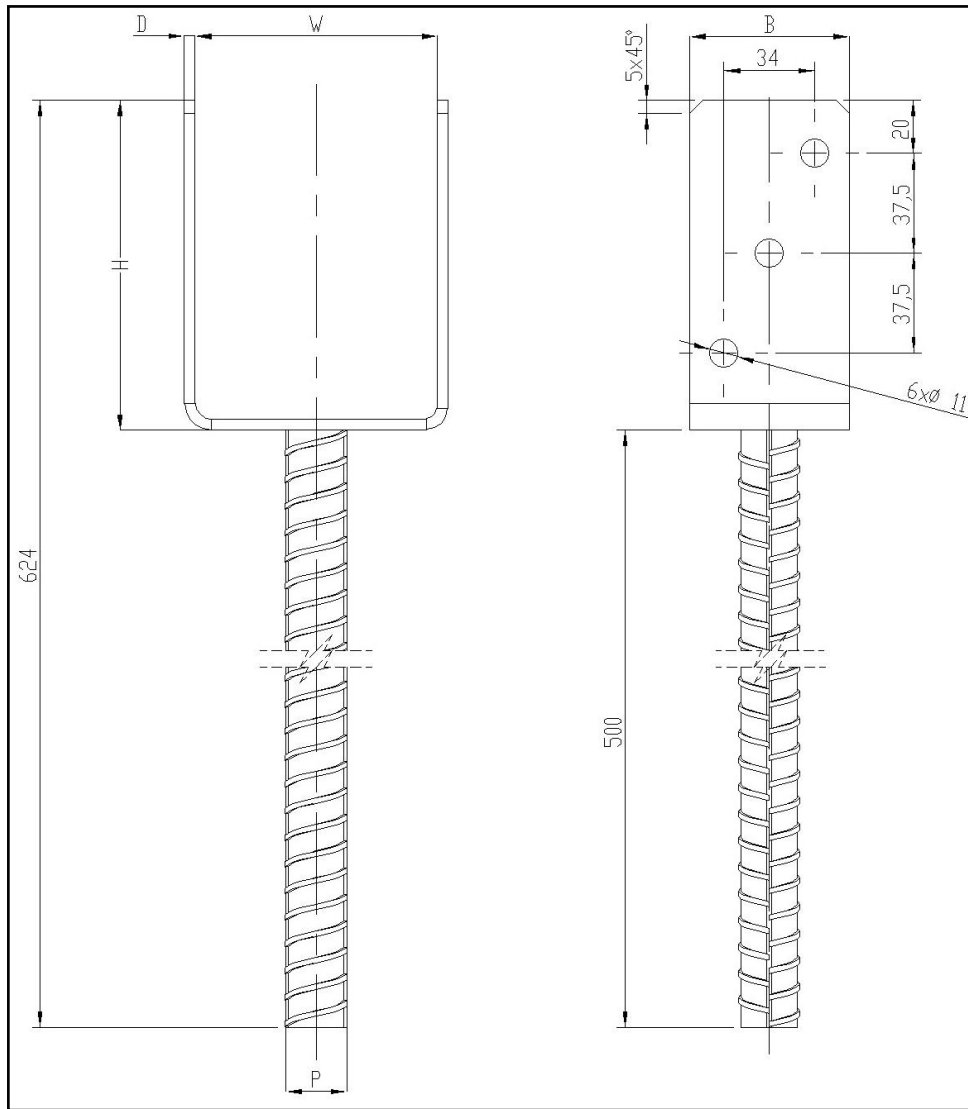
Figure 25 Type PS /500
