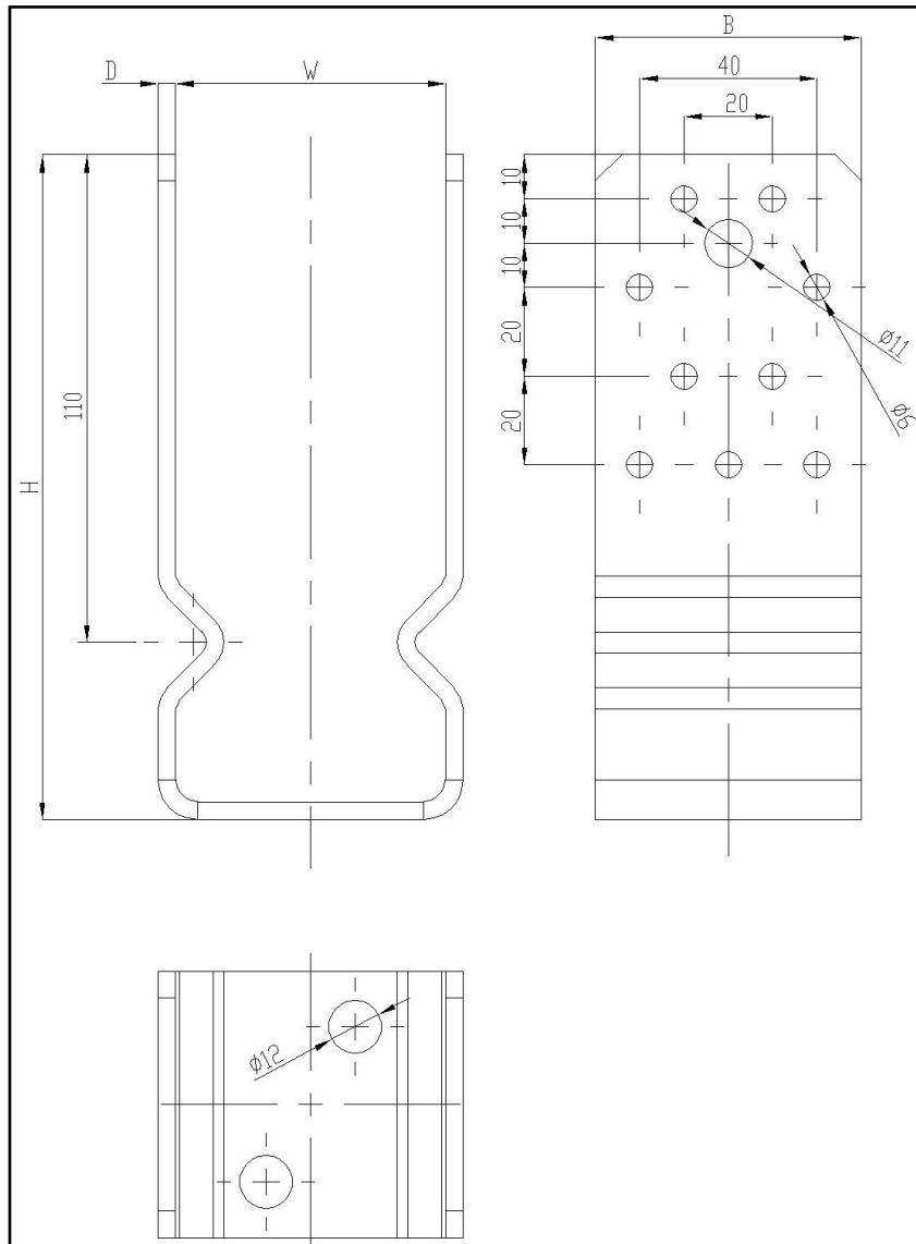
Figure 26 Type PSSOZ
