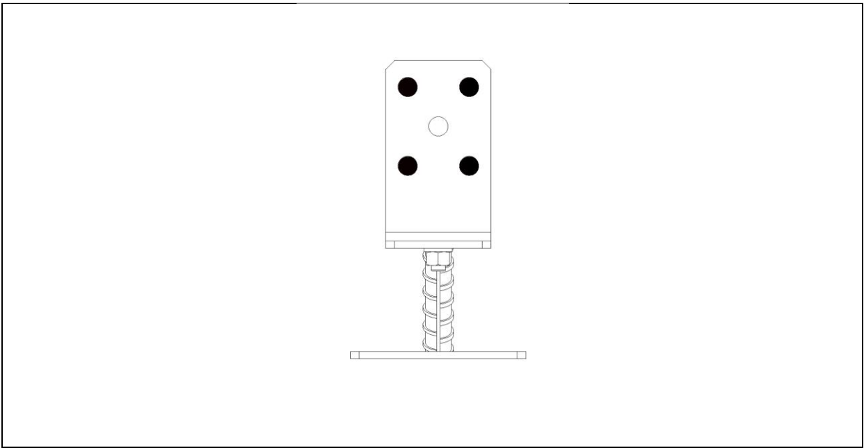
Figure 83 PSRLT 0-160
