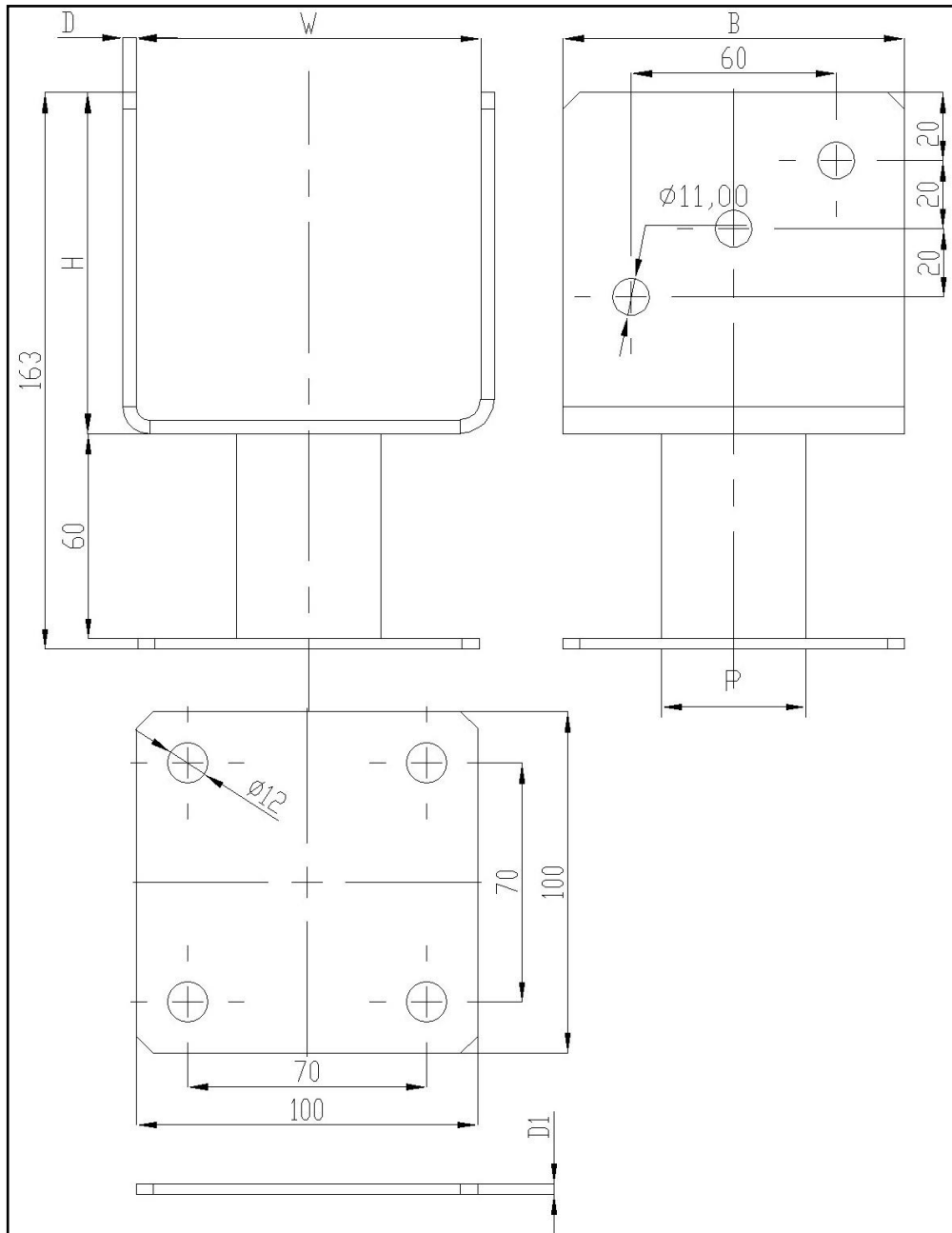
Figure 31 Type PMFU
