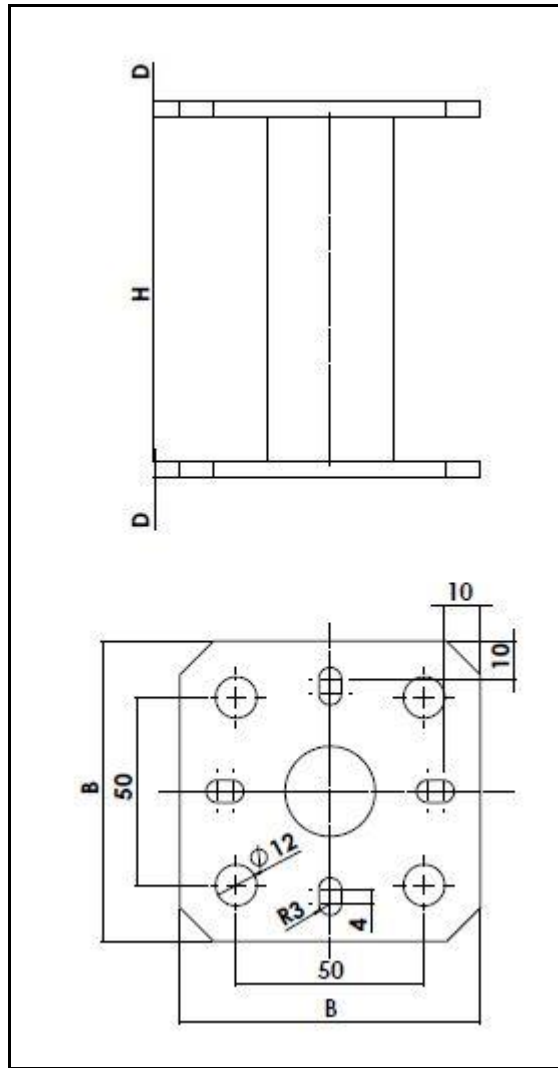
Figure 20 Type PMF 80-100
