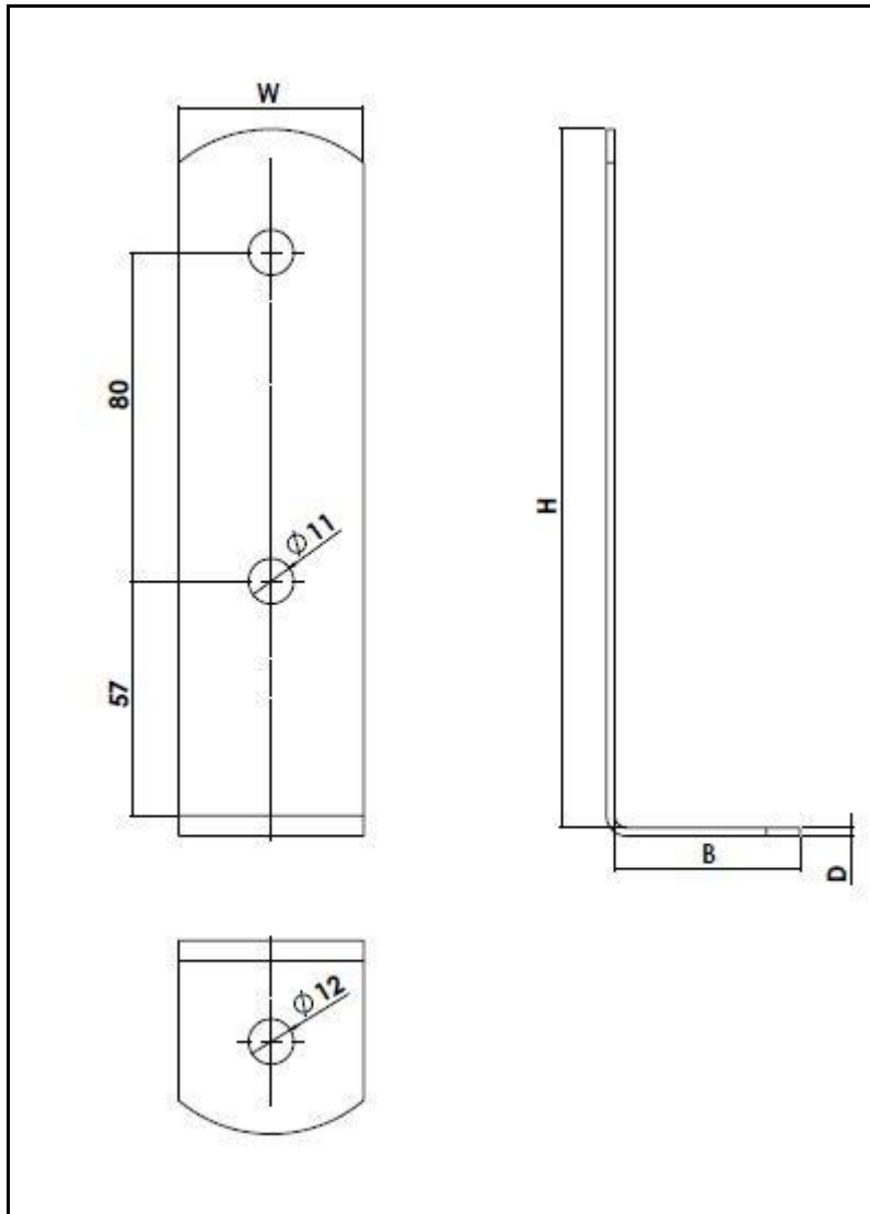
Figure 16 Type PSC 45
