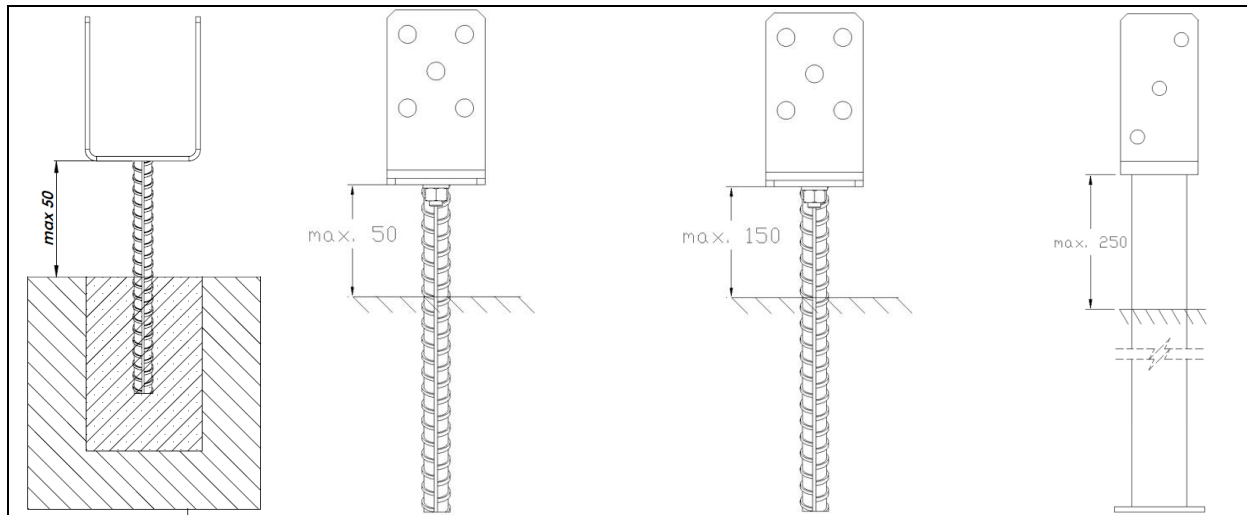
Figure 1 Post base with threaded rod
