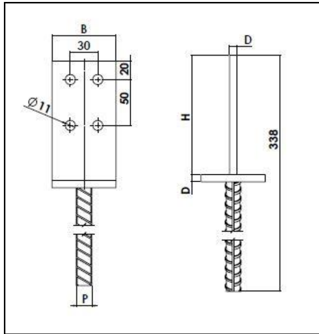
Figure 14 Type PSW 70
