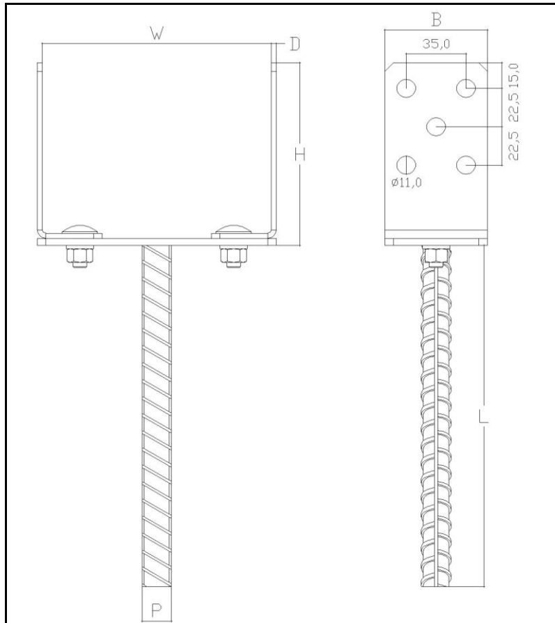
Figure 21 Type PSRL 0-160
