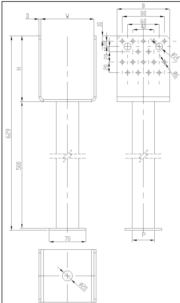
Figure 30 Type PSS R500
