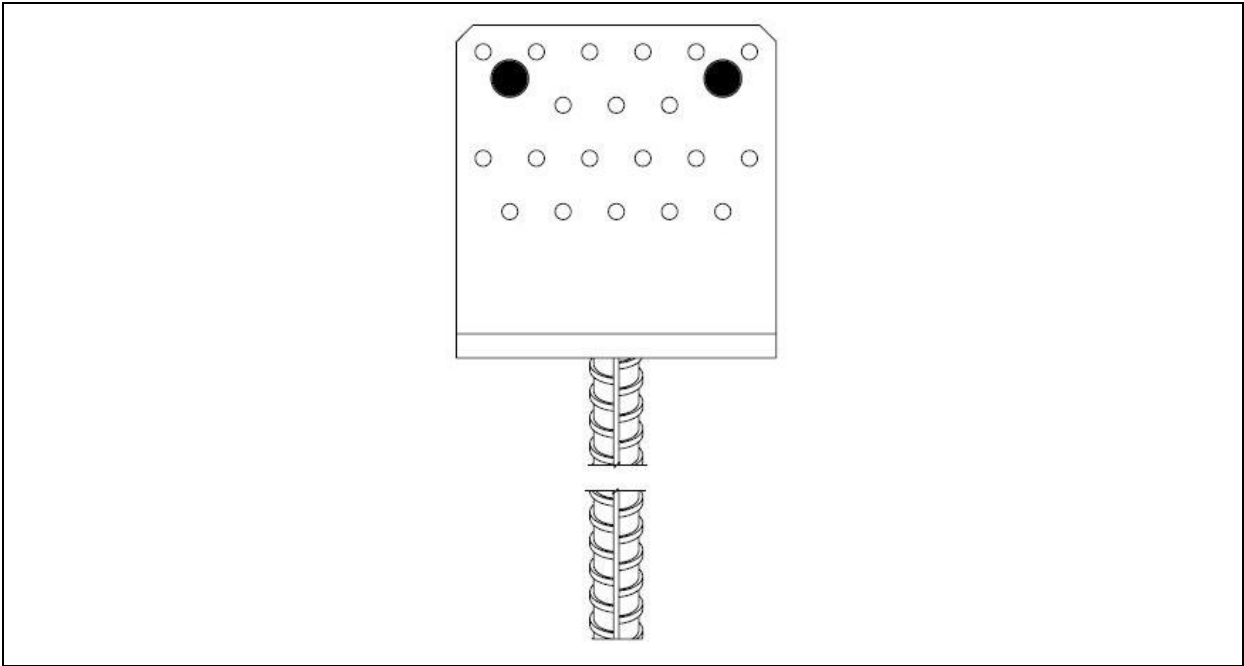
Figure 77 Type PSS 100, PSS 120, PSS 140
