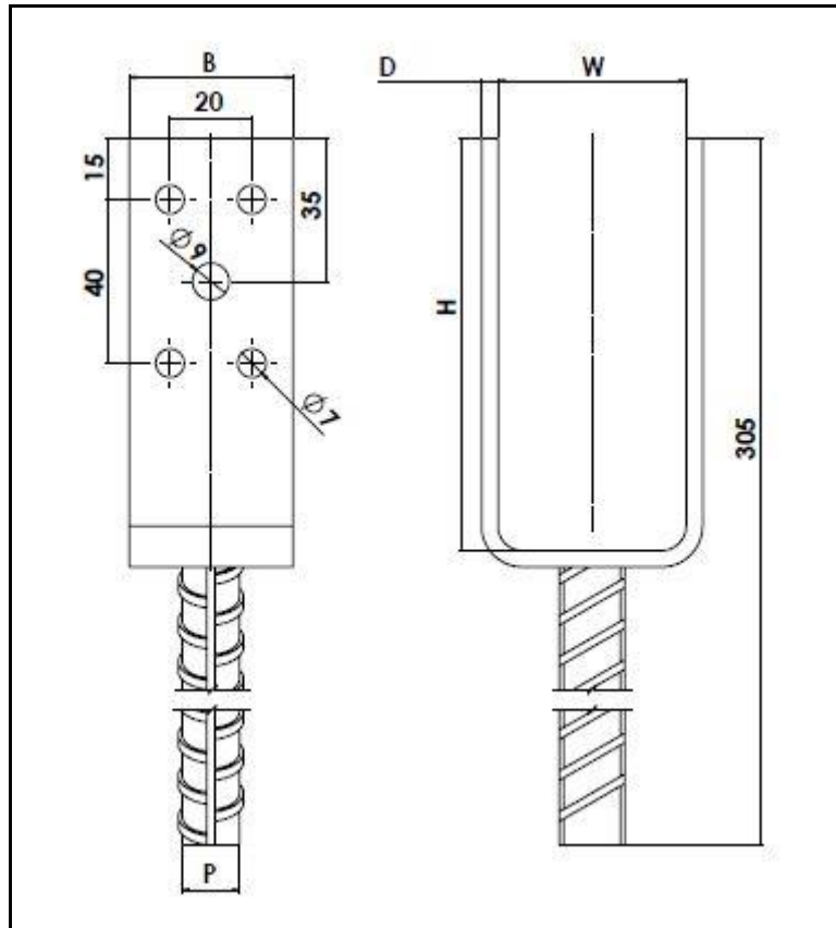
Figure 3 Type PSL 45U
