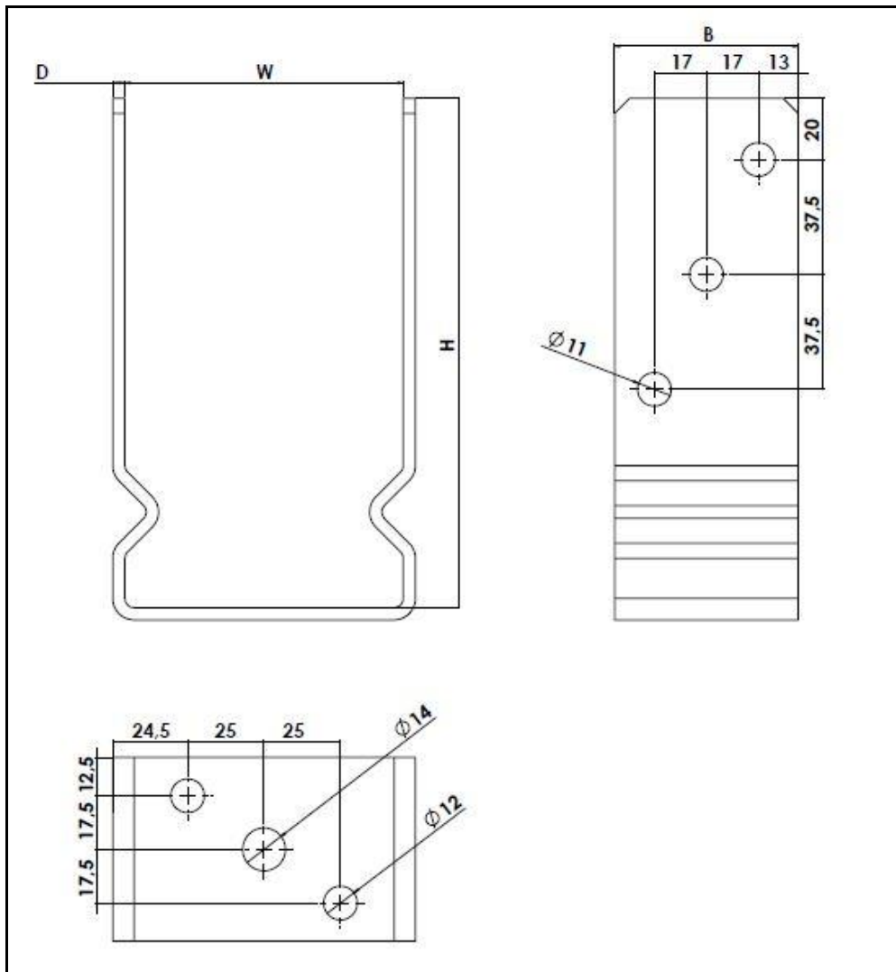
Figure 18 Type PSOZ 90
