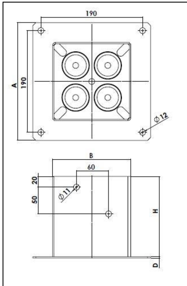
Figure 6 Type PSP 140
