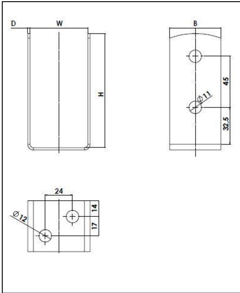
Figure 17 Type PSOL 50
