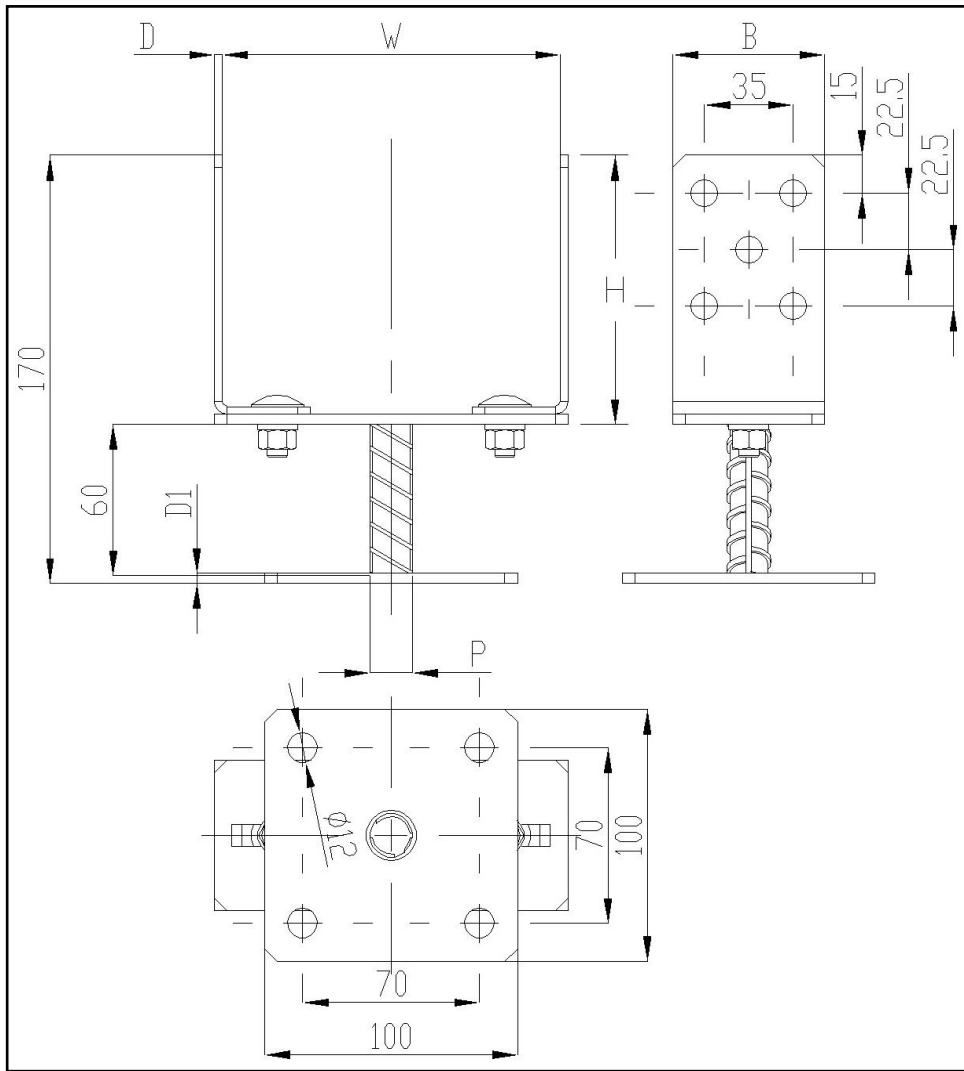
Figure 22 Type PSRLT 0-160
