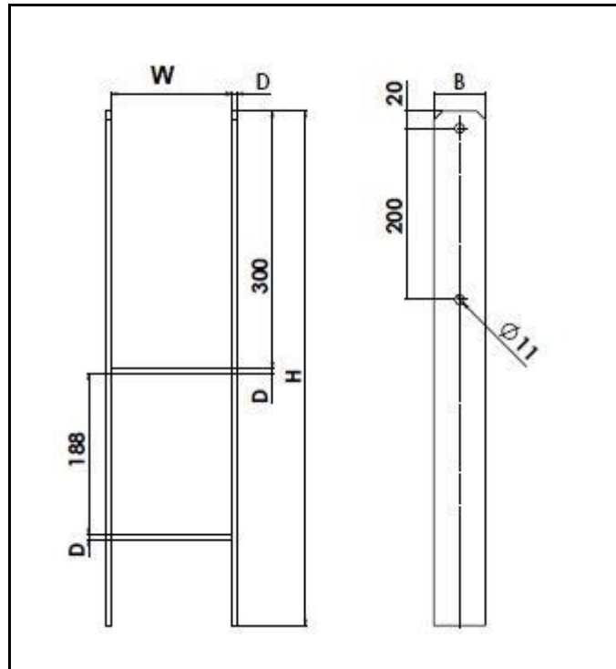
Figure 12 Type PSH 140
