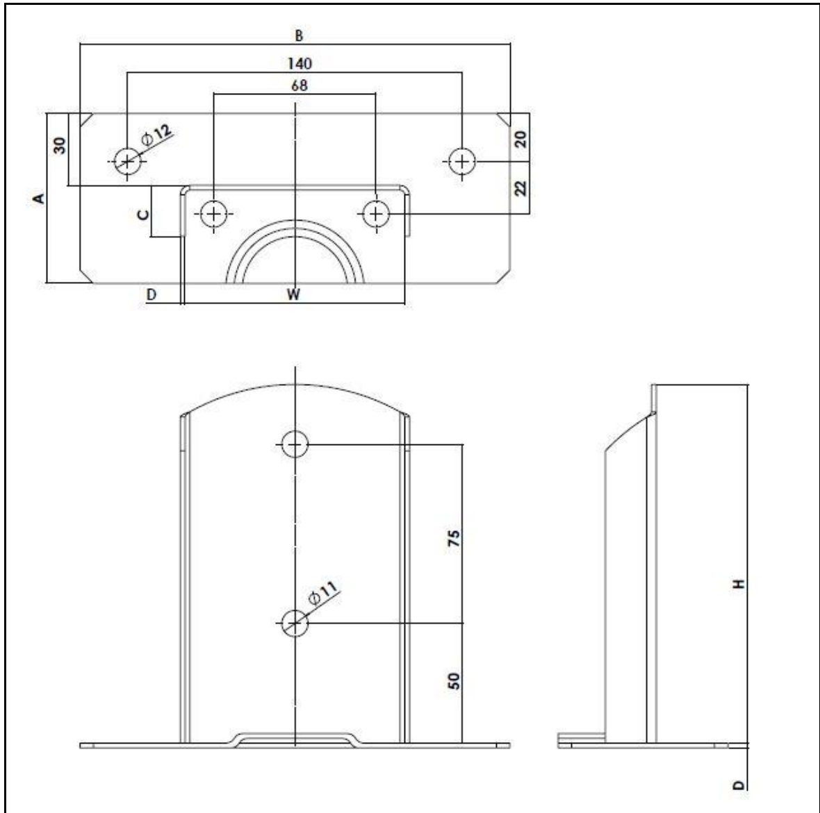
Figure 15 Type PSD 90
