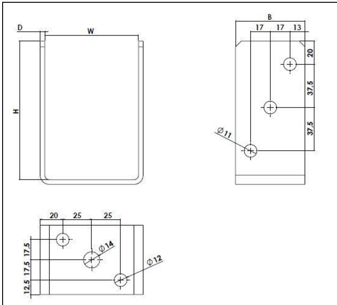
Figure 5 Type PSO 80
